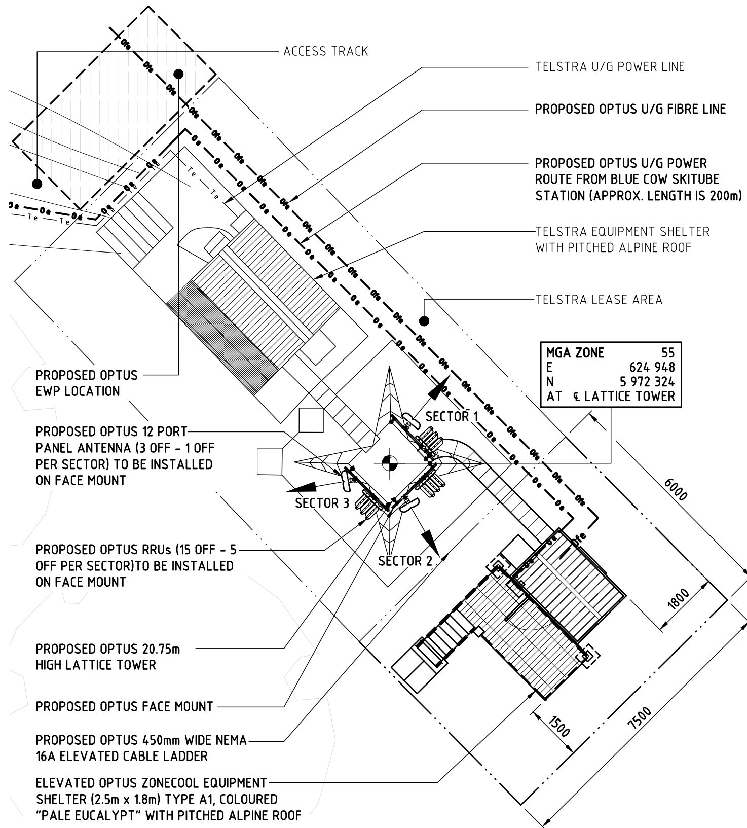
DETAIL 1 1:100
